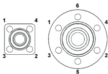
Tightening sequence
